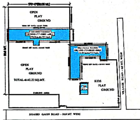
SITE PLAN
